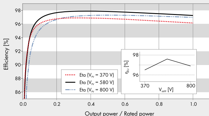
Efficiency curve SUNNY TRIPOWER 10000TL
